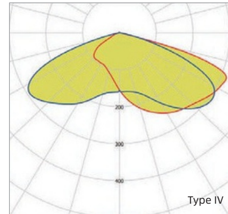
Large light distribution
